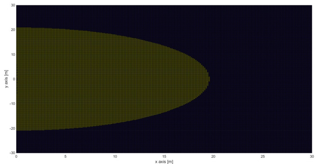
Figure 21. Area of electric field strength with values higher (yellow) and lower (blue) than the limit of 1.25\text{ V/m} for method “C” of linear current source for a linear frame of 13 electrodes with D_{el} = 1.0\text{ m} for the area of Korakia ( \rho_S = \infty , without dam, L = 1.1815\text{ m} , \rho_w = 0.25\ \Omega\cdot\text{m} , \theta = 248^\circ , J_{maintenance\_steady} = 22\text{ A/m}^2 ).
