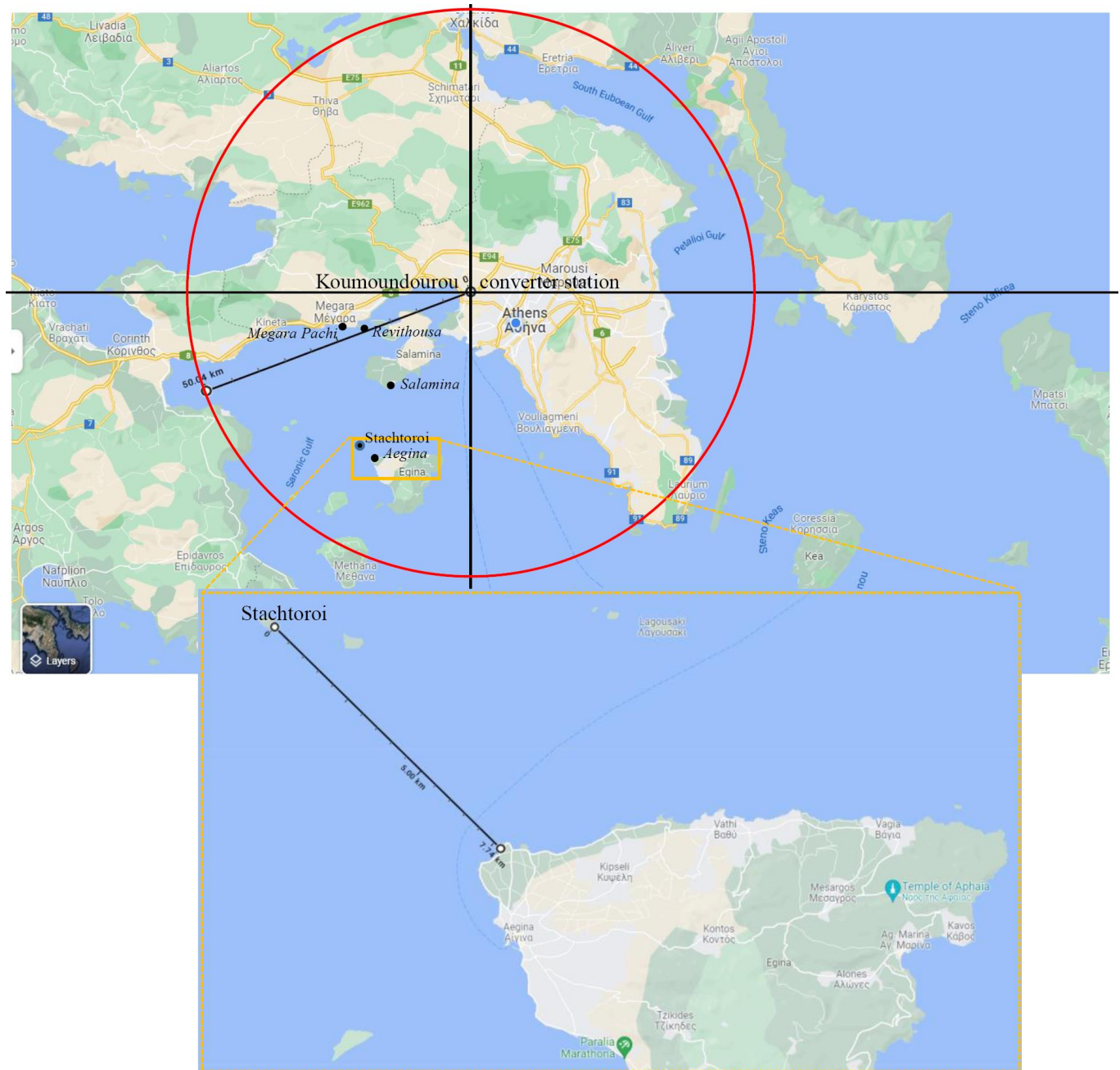
Figure 2. Location of the electrode station for an HVDC transmission system in the region of Attica–Stachtroi (with italics are the nearby residential areas under study).
