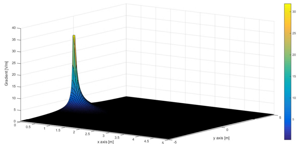
Figure 18. Electric field strength for method “C”, of linear current source, for the area of Korakia ( \rho_s = \infty , without dam, L = 1.1815 \text{ m} , \rho_w = 0.25 \Omega\cdot\text{m} , \theta = 248^\circ , J_{\text{maintenance\_steady}} = 22 \text{ A/m}^2 ).
