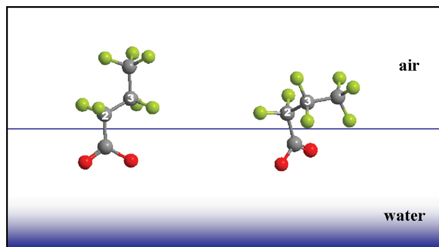
Figure 5. Anti perfluorobutanoate (left) and gauche -perfluorobutanoate (right) at the air/water interface. A closer approach of fluorine atoms to the water surface minimizes the free energy of the system. 52,67,71
