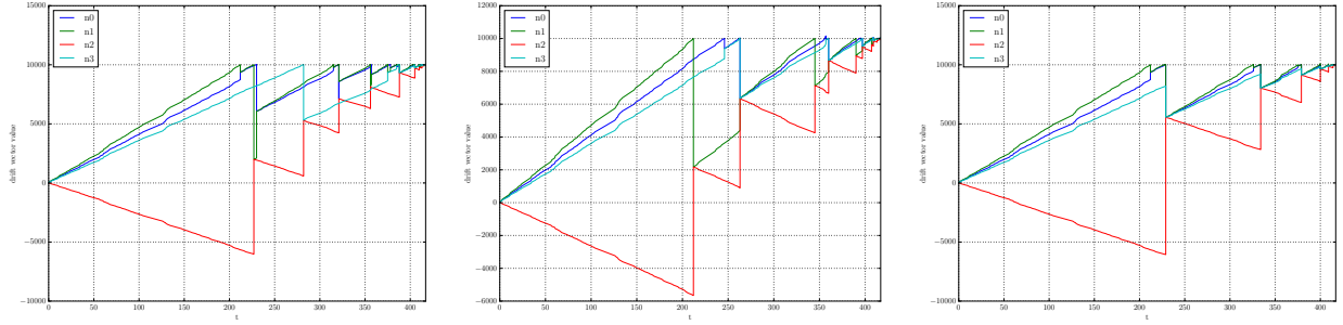
(a) Drift vectors of 4 nodes as a result of the GM method. (b) Drift vectors of 4 nodes as a result of the DIST method. (c) Drift vectors of 4 nodes as a result of the DISTR method.
