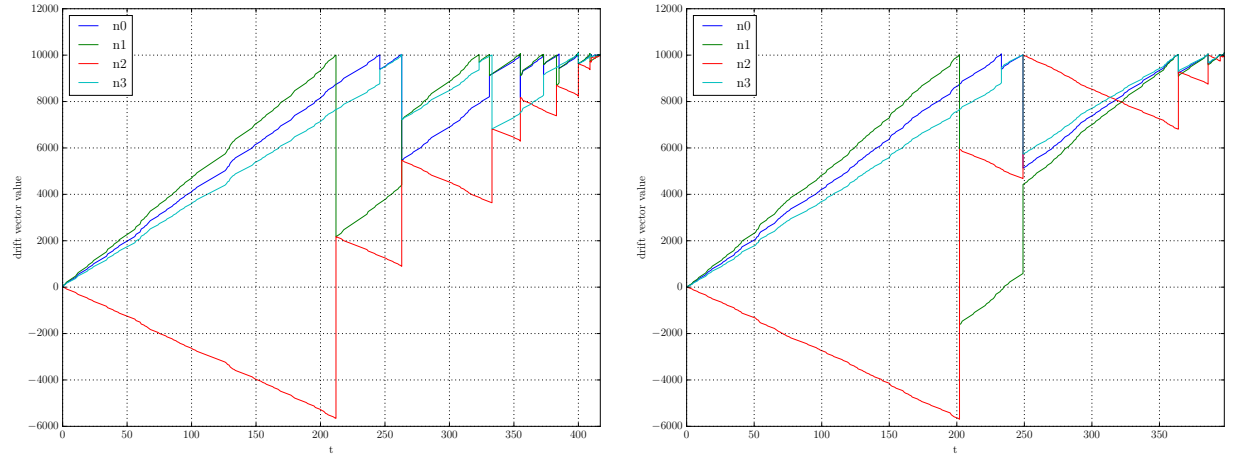
(a) Drift vectors of 4 nodes, as formulated by the GM algorithm. (b) Drift vectors of 4 nodes, as formulated by the HDM algorithm.
