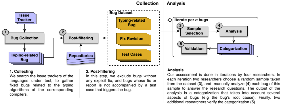
Fig. 1. The overview of our bug collection and bug analysis approach.
