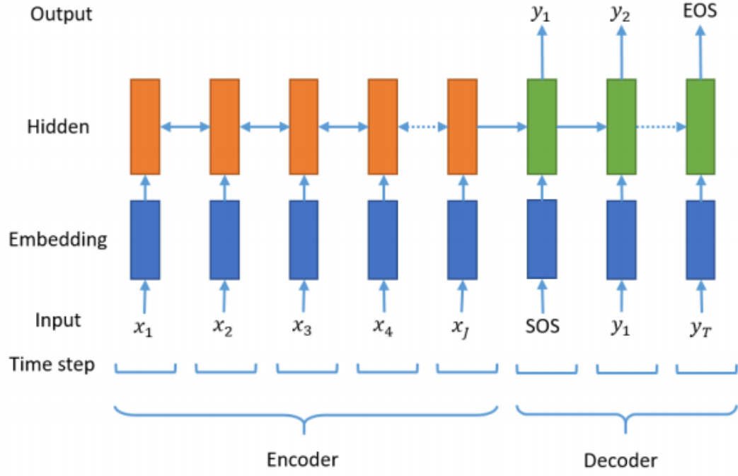
Figure 3.1: Single Document Text Summarization Model [53]
