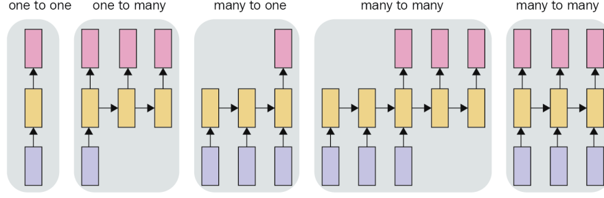
Figure 2.1: Various RNN design patterns [23]
