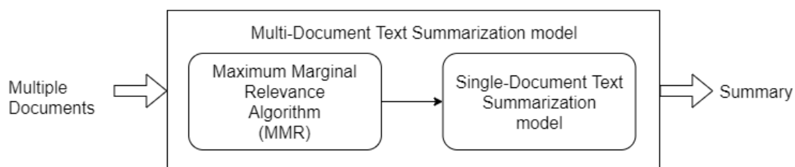
Figure 5.1: PG-MMR multi-document text summarization model
