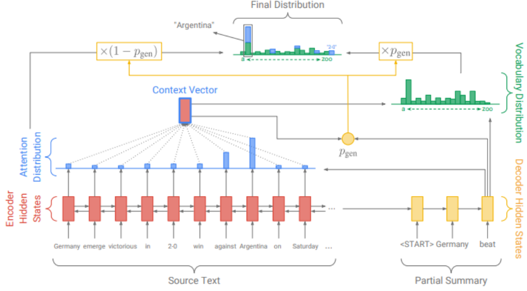
Figure 3.3: Pointer generation mechanism on Single Document Text Summarization Model [52]
