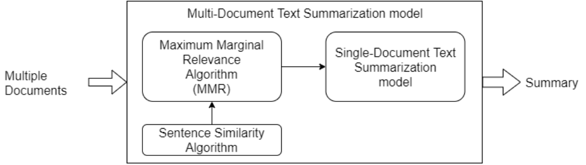
Figure 5.3: PG-MMR-SS multi-document text summarization model
