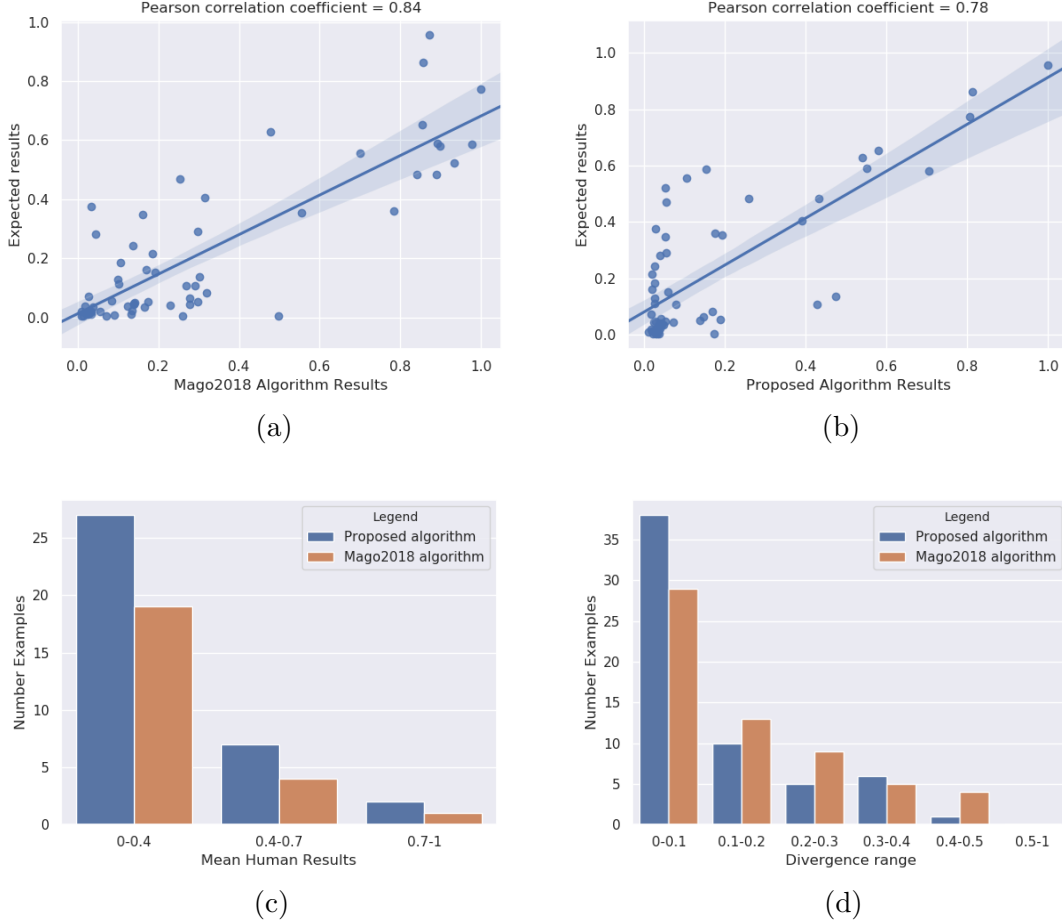
Figure 6.1: Pearson correlation coefficients and statistical measurements between algorithms.
