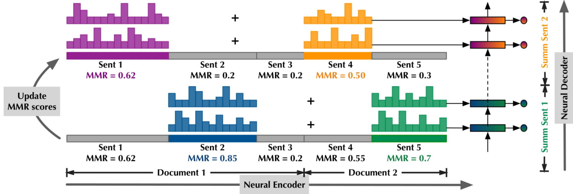
Figure 5.2: “Muting”attention mechanism on Maximal Marginal Relevance Algorithm [49]
