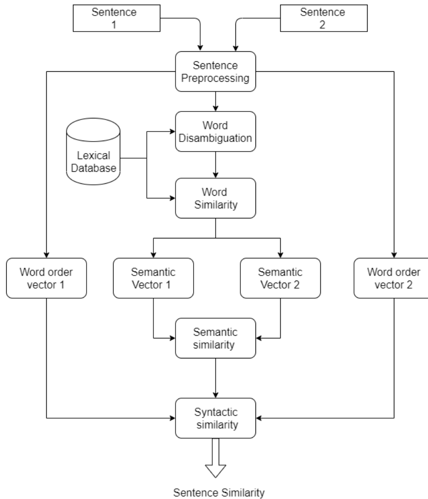
Figure 4.1: Proposed sentence similarity algorithm
