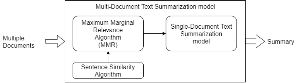
Figure 1.1: The State-of-the-art multi-document text summarization model with our proposed sentence similarity algorithm
