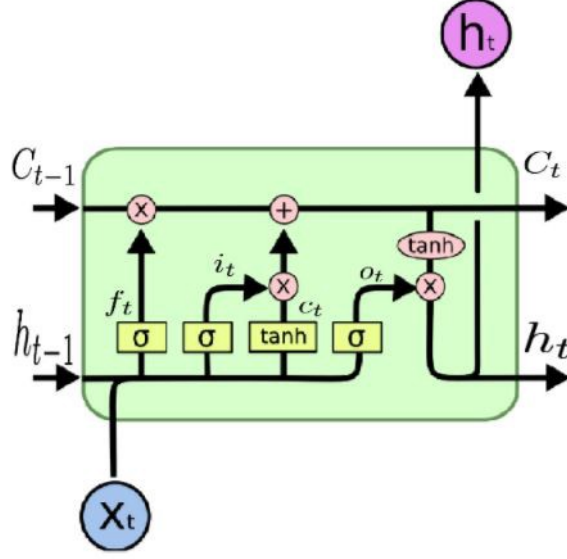
Figure 2.2: The LSTM cell [40]
