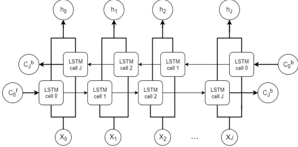
Figure 2.3: Bidirectional Long Short Term Memory network
