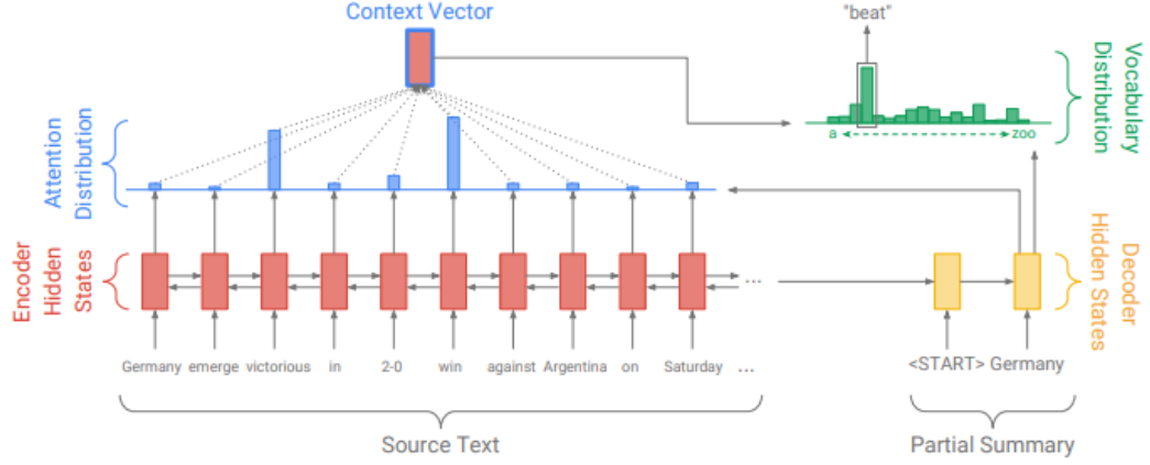
Figure 3.2: Attention mechanism on Single Document Text Summarization Model [52]
